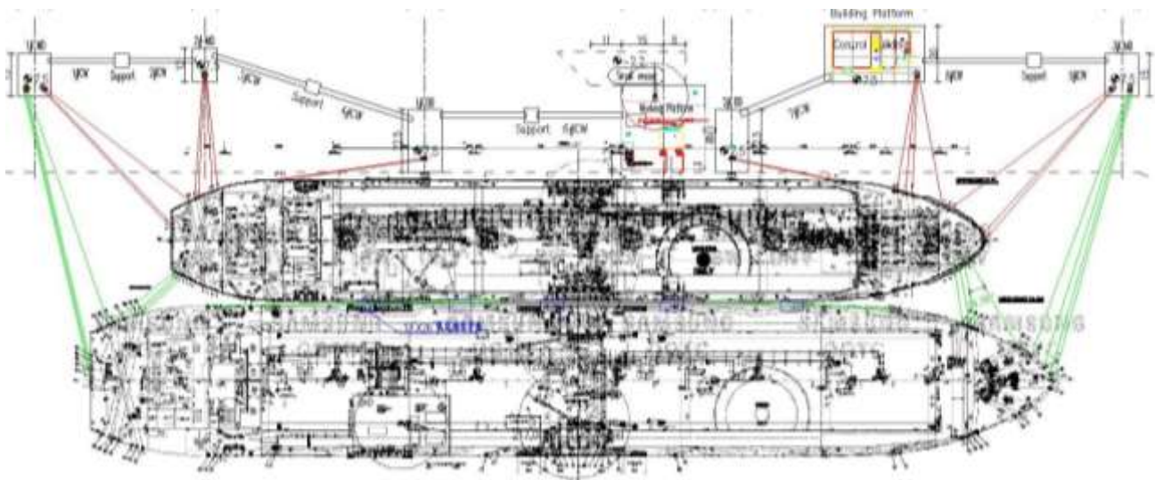
Figure 5–Terminal Mooring Layout
