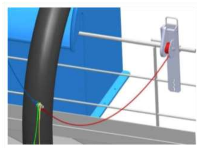
Figure 17: LNGC SWPS connection
